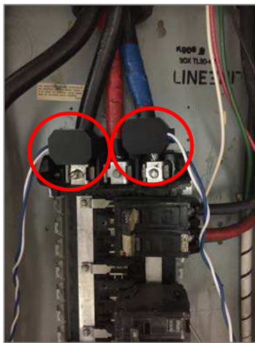
Two Consumption Metering Current Transducers
